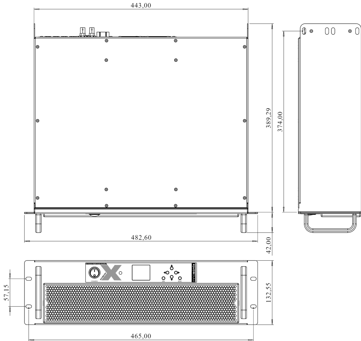
Figure 1. MAXX/HP 2 dimensions
